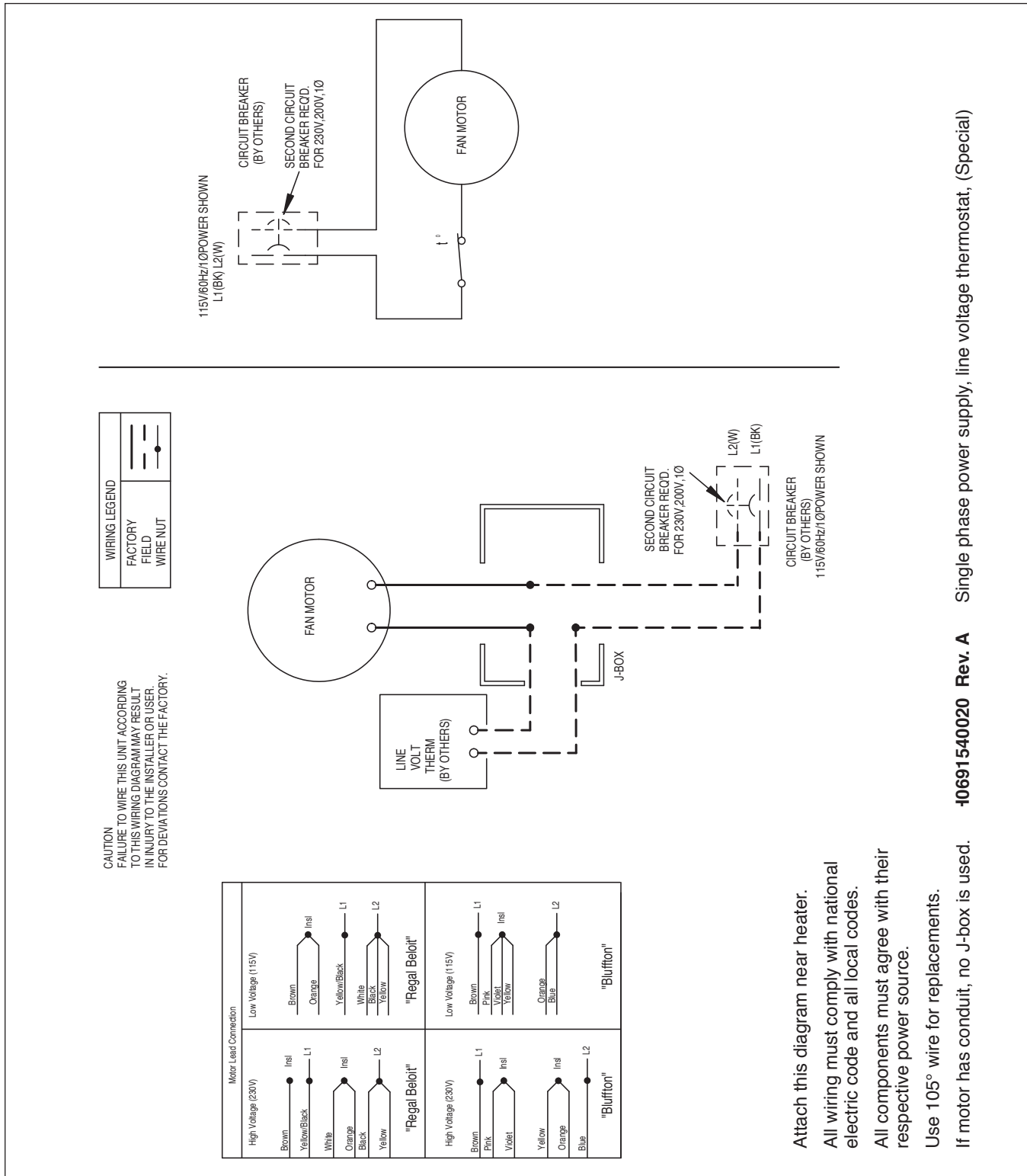
Figure 2 Steam/Hot Water Unit Heater Wiring Diagram - 115V/1ph (V/VN, PT/PTN, WVC/MVW, WPC/WPN 333 only)
